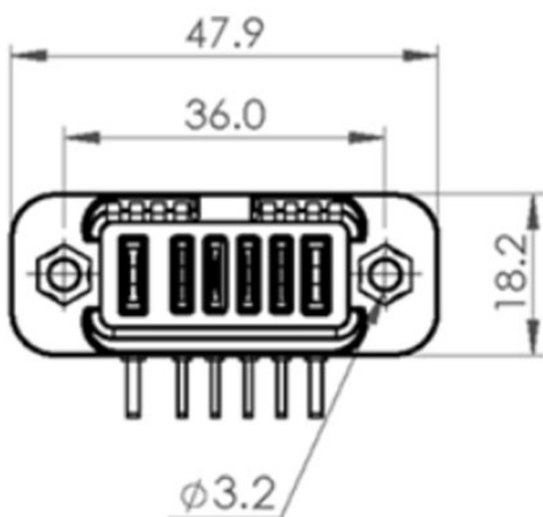
Male Connector
