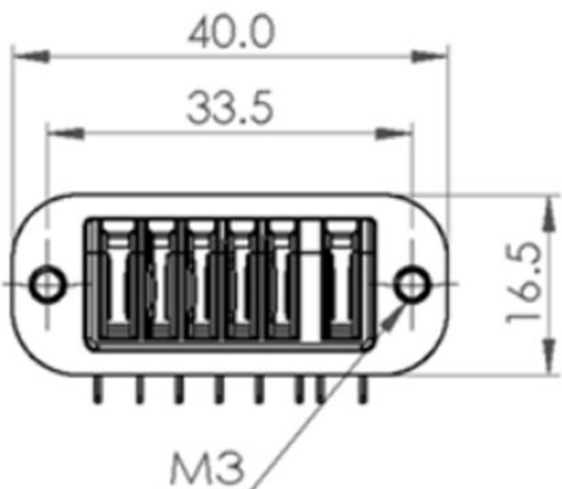
Female Connector
